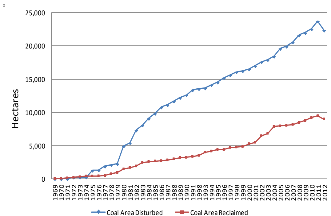
Figure 7: Area Disturbed and Reclaimed by Coal Mines in B.C. (1969–2012)
